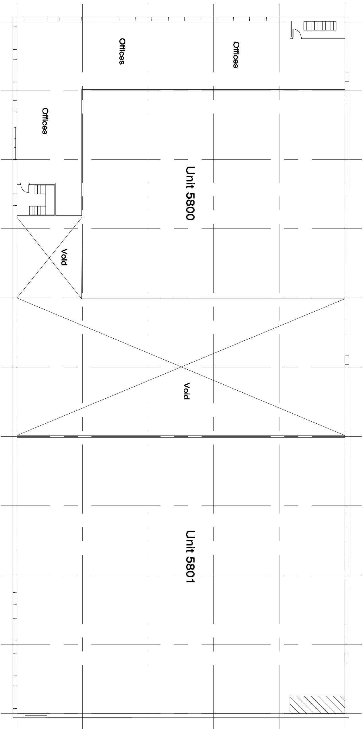
First Floor Plans of Units 5800 & 5801 Scale 1:200
