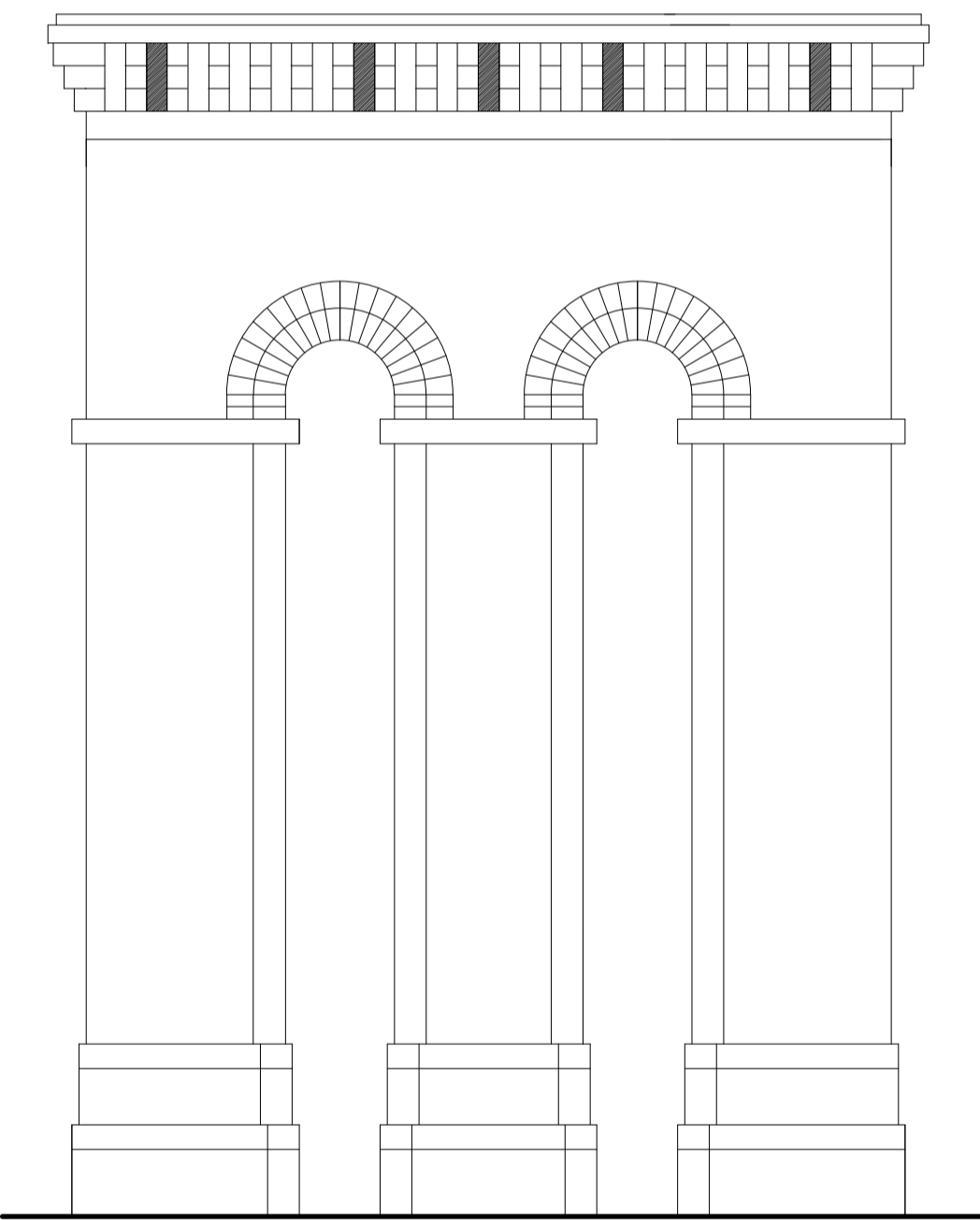
side / south elevation
