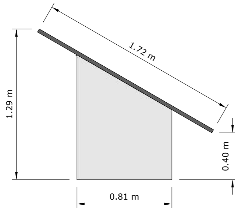
Panel Side Elevation (1:20)
