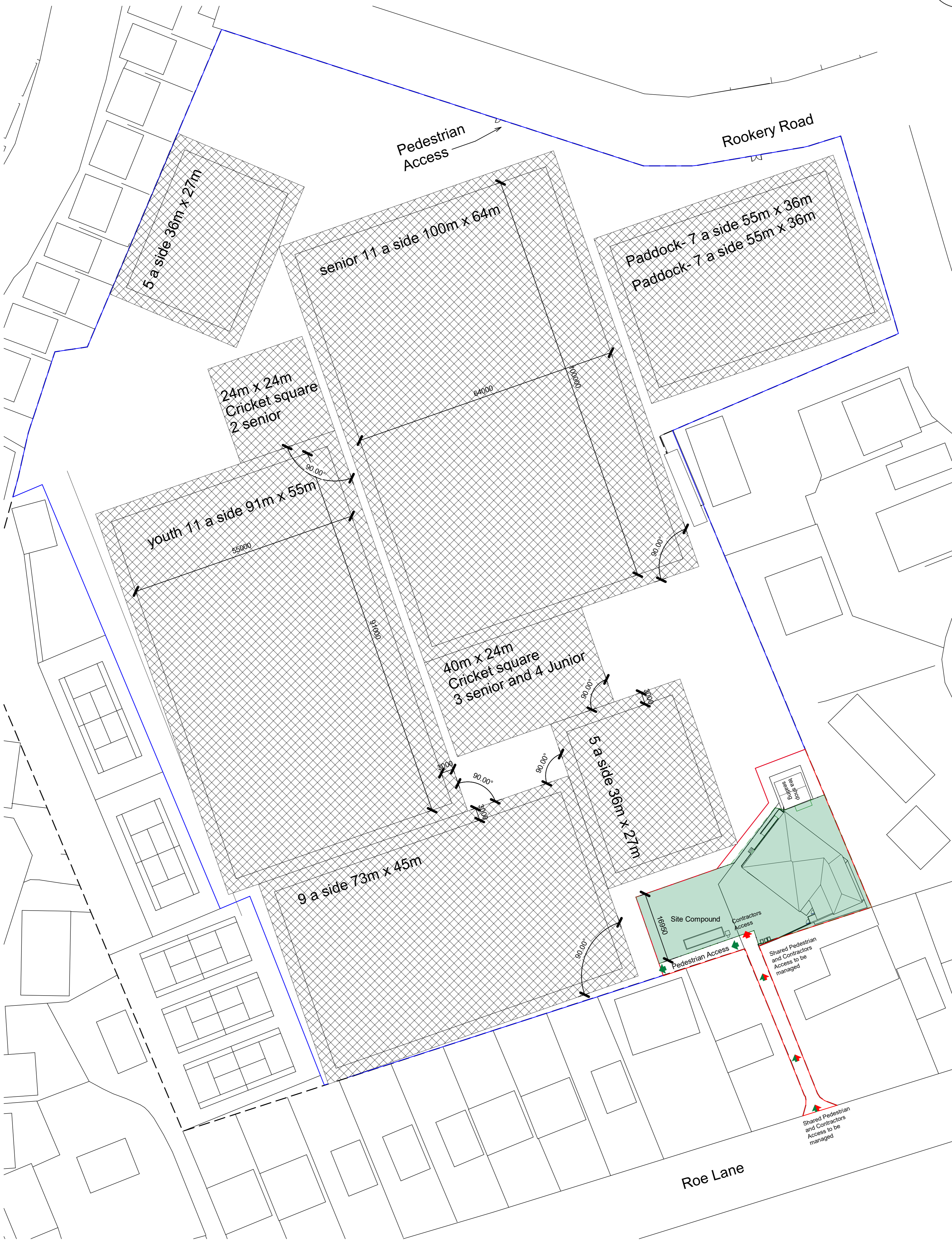
1 Site Compound 1 : 500
