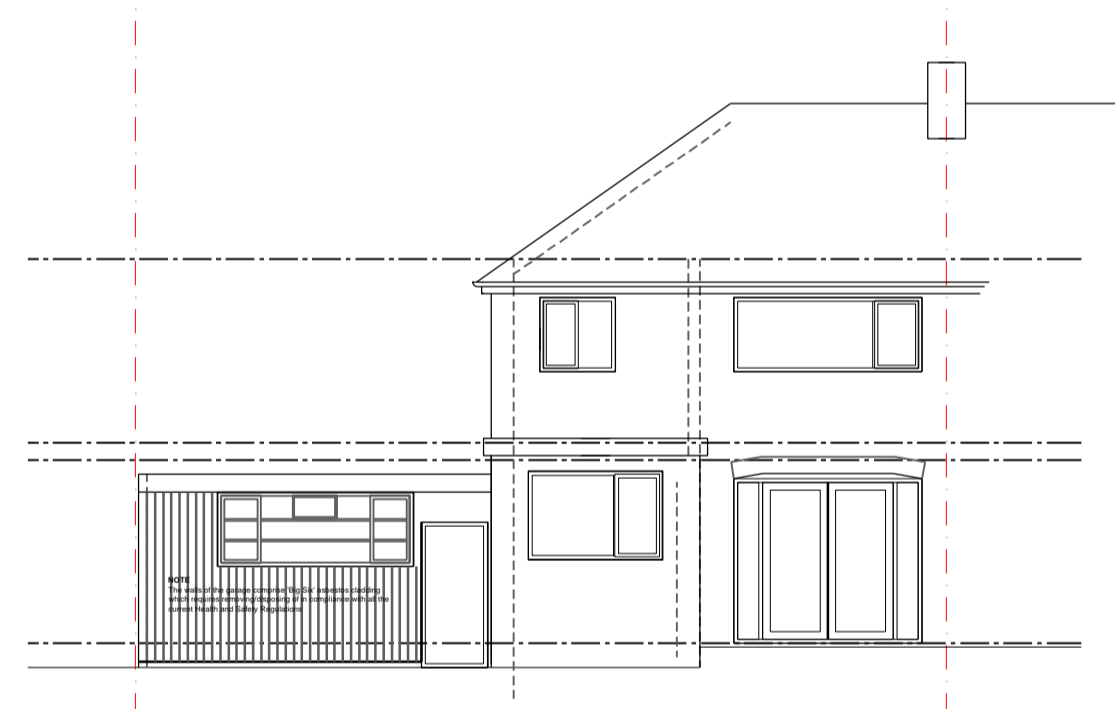
EXISTING REAR ELEVATION | 6 FD 0H
