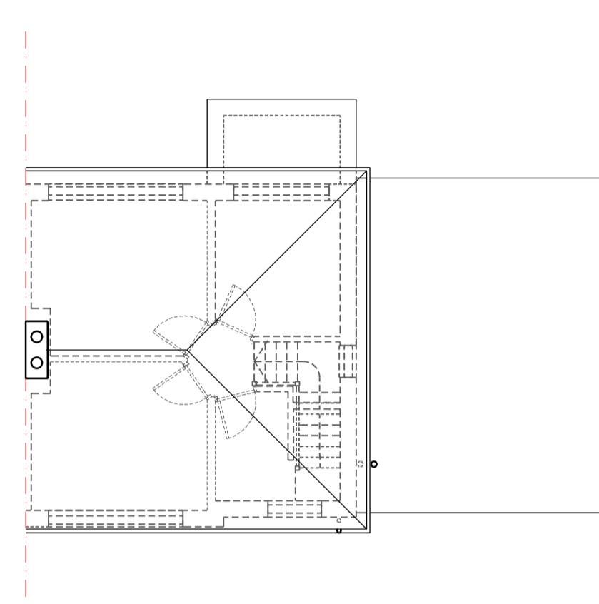
EXISTING ROOF PLAN | 6 FD 0H
