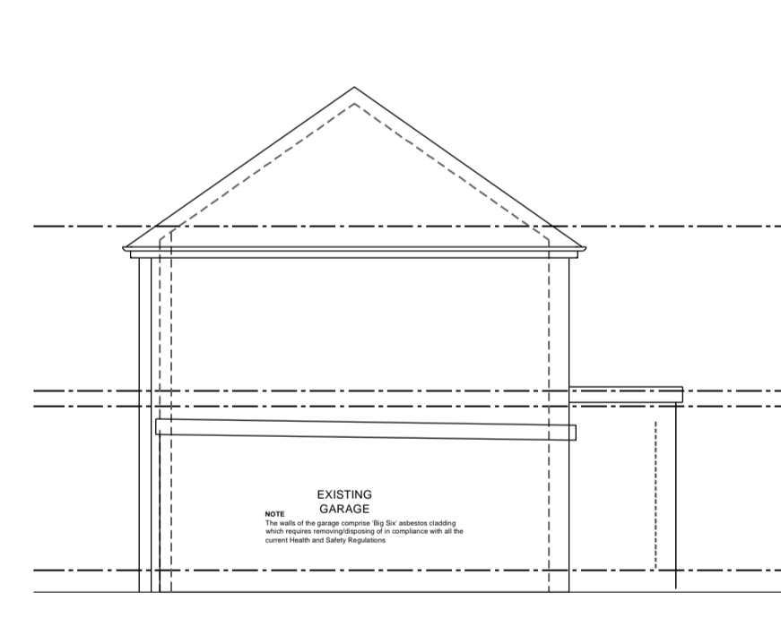
EXISTING SIDE ELEVATION 01 | 6 FD 0H
