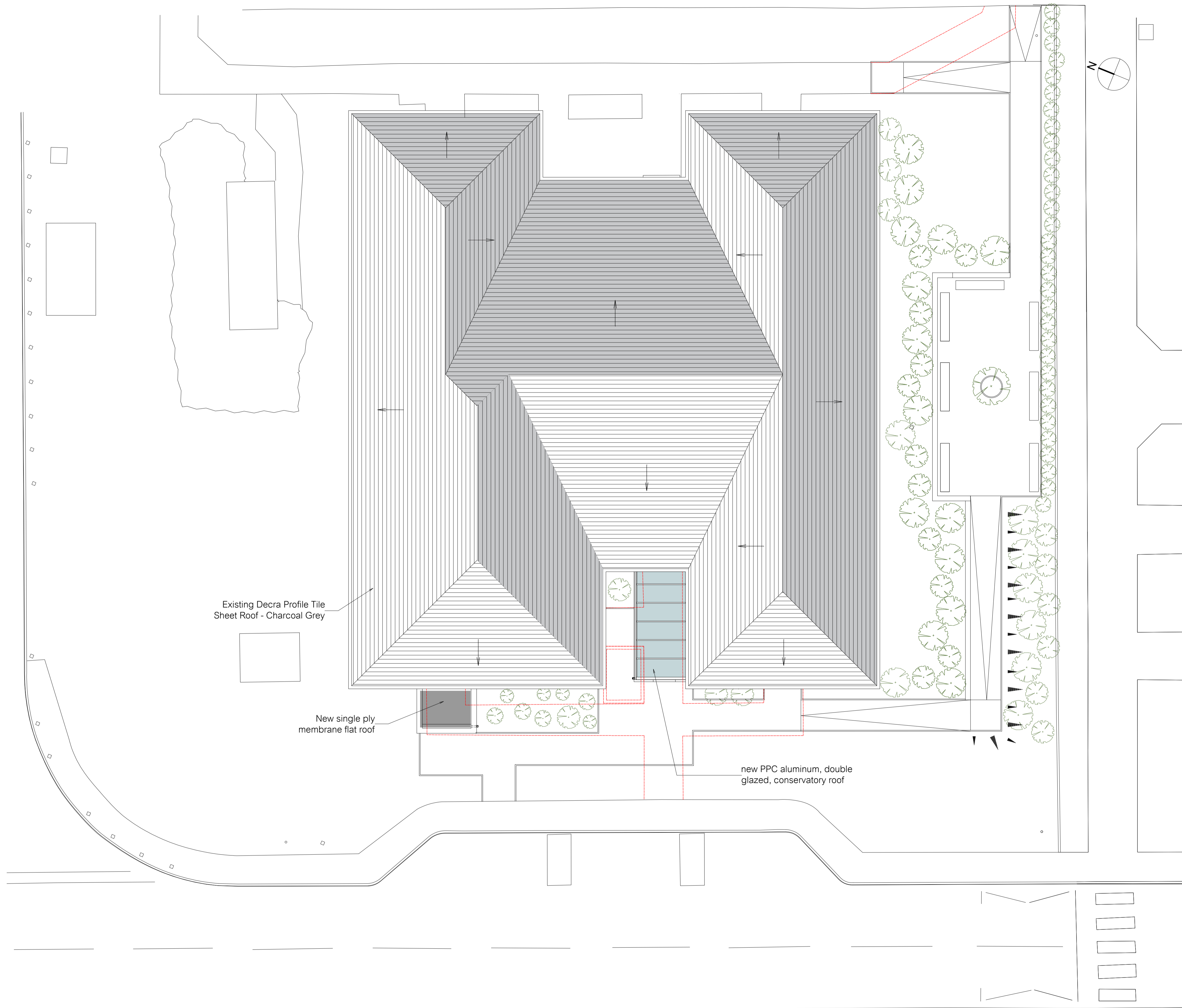
Proposed Roof Plan Scale 1:100
