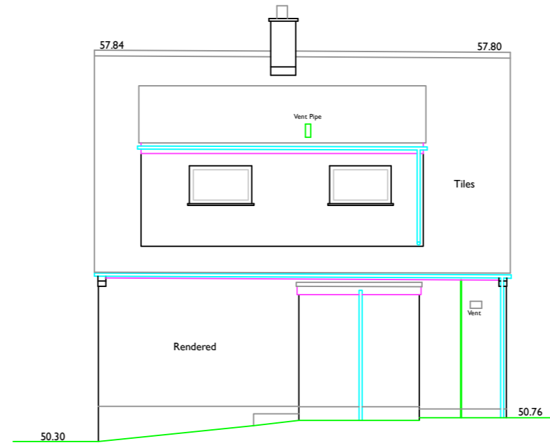
EXISTING NORTH EAST/ SIDE ELEVATION 2
