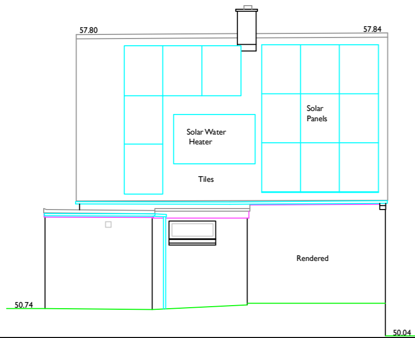
EXISTING SOUTH WEST/ SIDE ELEVATION 4
