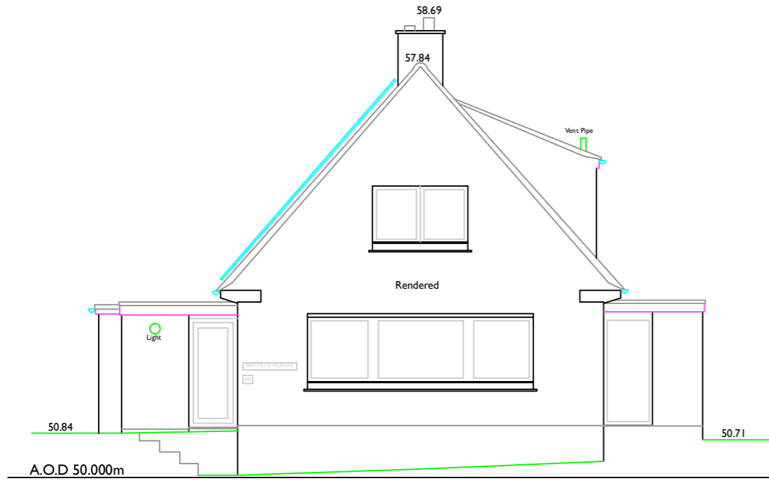
EXISTING SOUTH EAST/ FRONT ELEVATION 1
