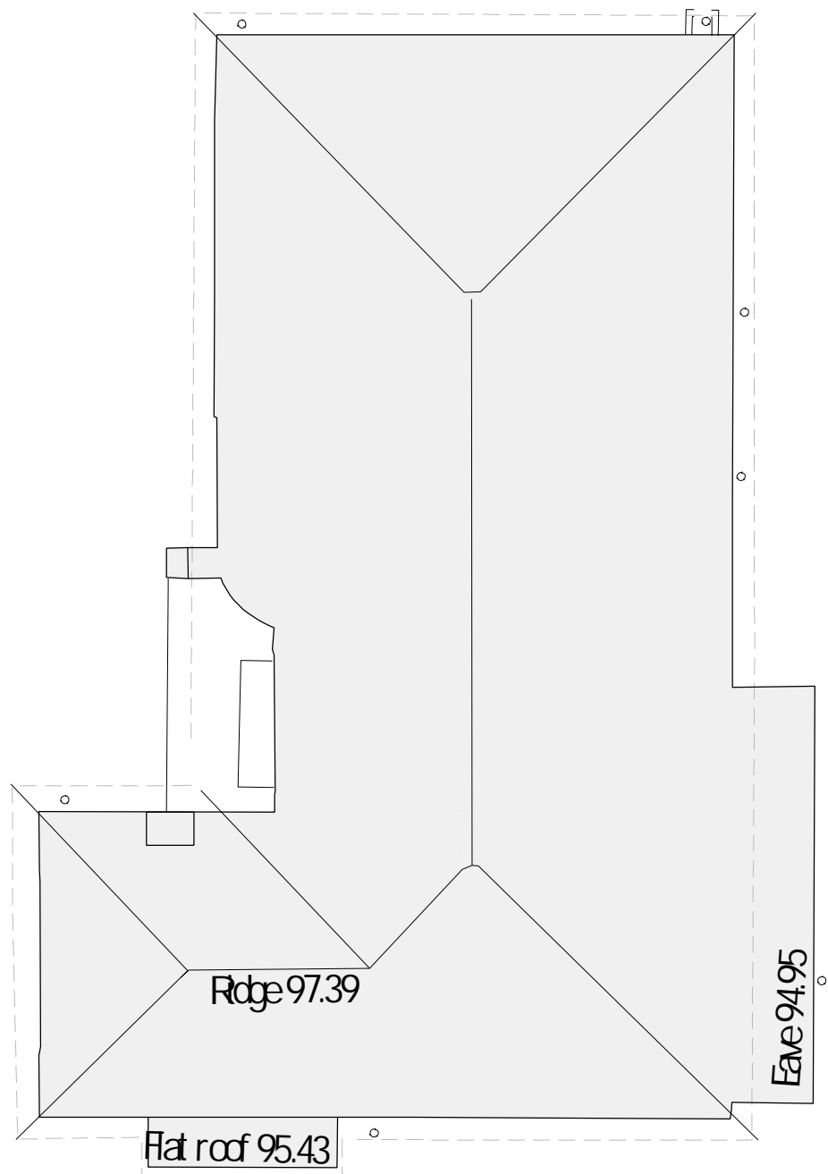
01 ROOF PLAN
