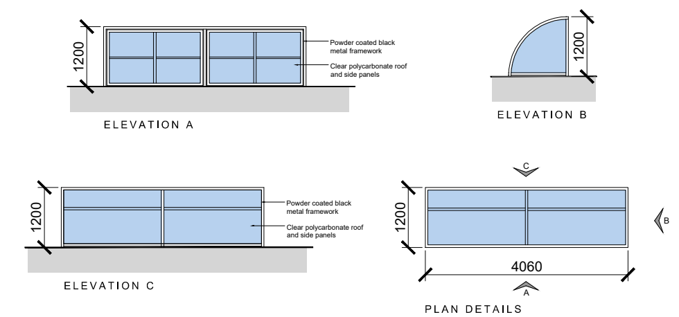
2 PROPOSED BUGGY STORE 1:100
