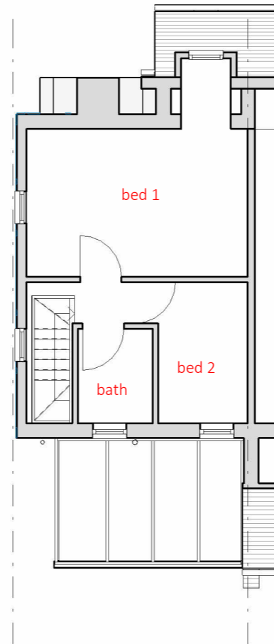
2 P01 P4.0 First Floor as existing 1 : 100
