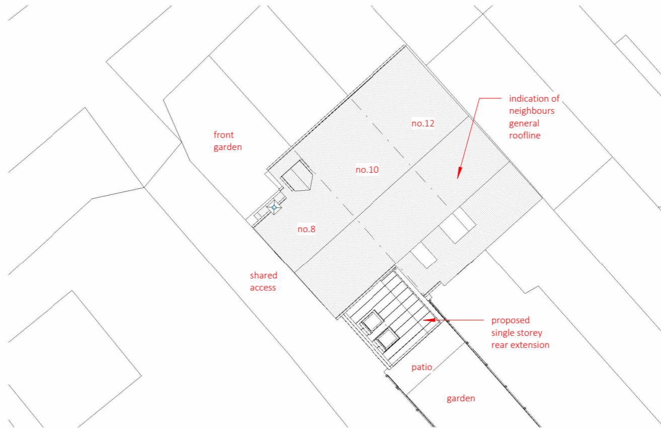
5 P01 P2.0 Block Plan as proposed 1 : 200
