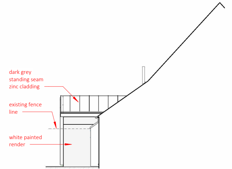
7 P03 north east elevation as proposed 1:100
