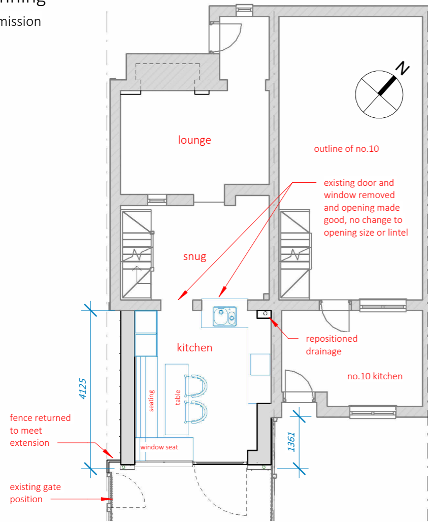
1 P03 P3.1 Ground floor as proposed 1:100
