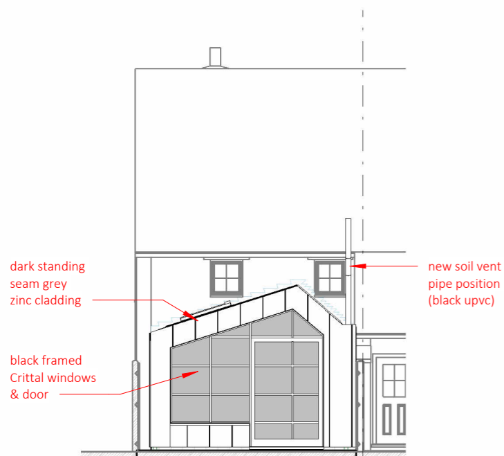
4 P03 south east elevation as proposed 1:100
