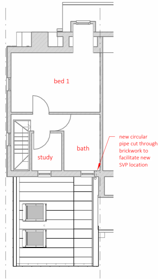
2 P03 P4.1 First Floor as proposed 1:100
