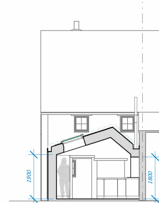
6 P03 Section AA proposed 1:100
