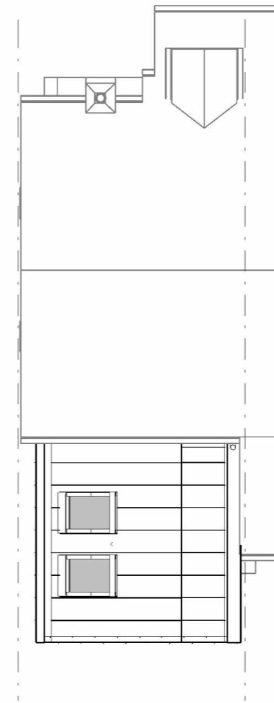
3 P03 P5.1 Roof Plan as proposed 1:100
