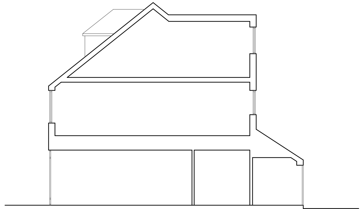
EXISTING SECTION
