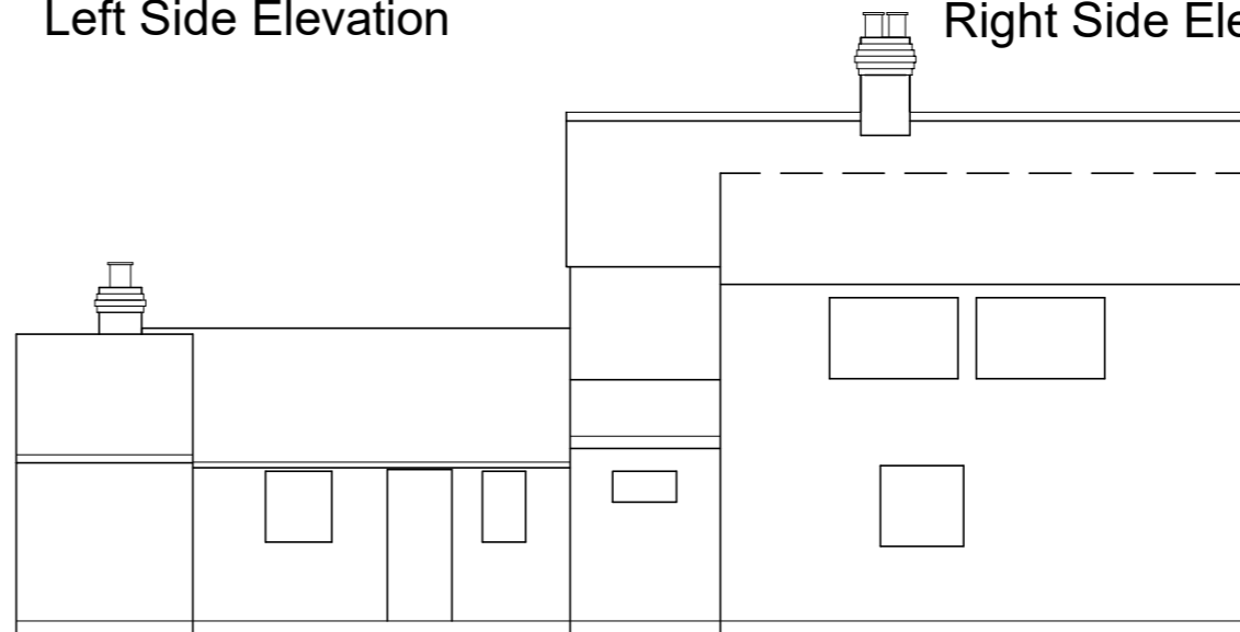
Rear Elevation
