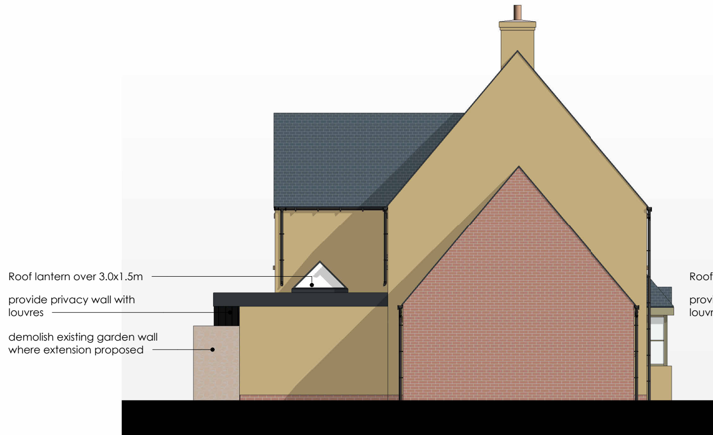
East Elevation
