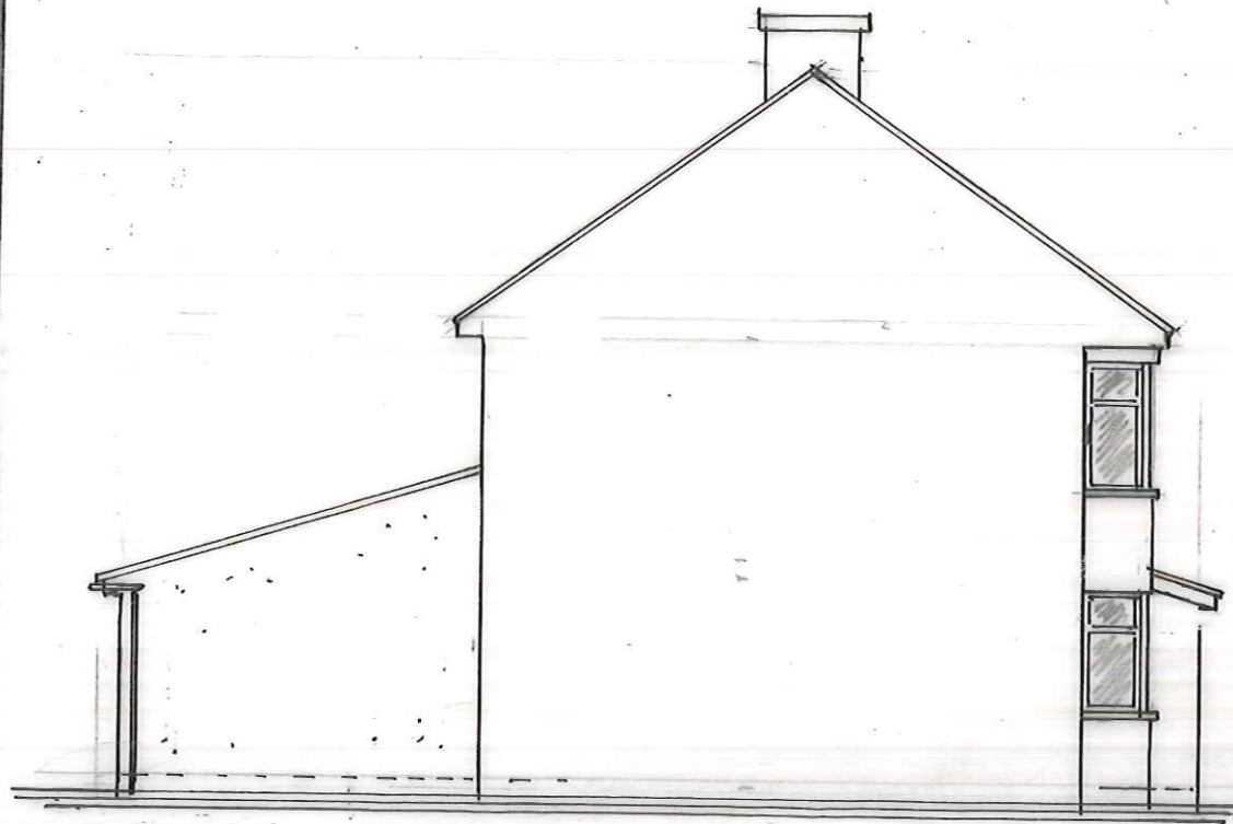
SIDE EL.
