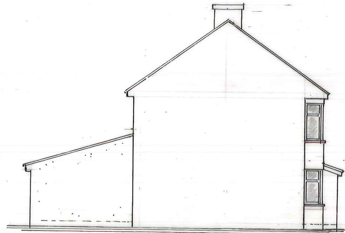
SIDE EL.
