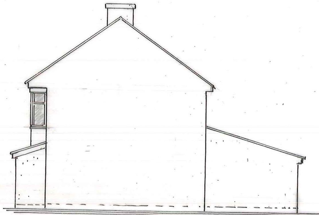
FLANK EL.
