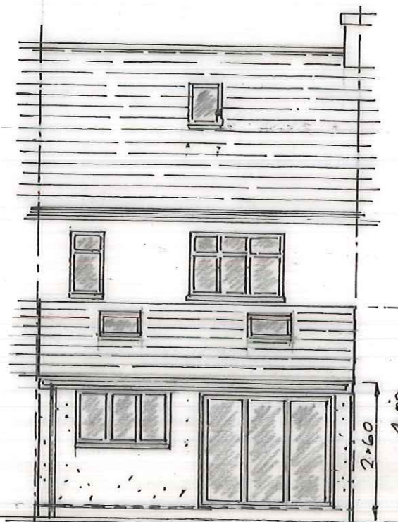
REAR EL.
