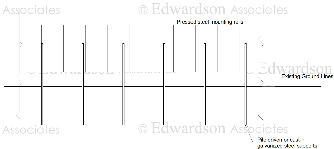
Elevation B (1:100)
