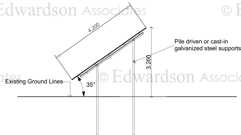
Elevation D (1:100)
