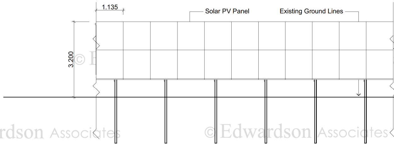
Elevation D (1:100)
