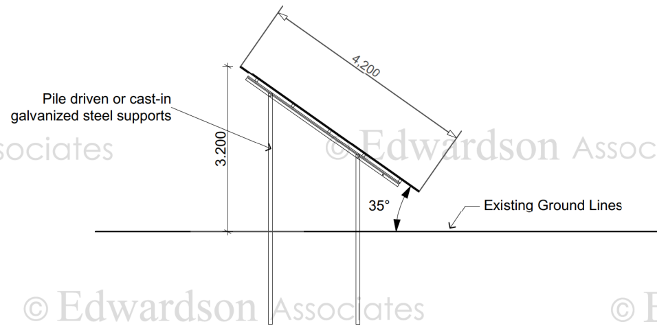
Elevation A (1:100)
