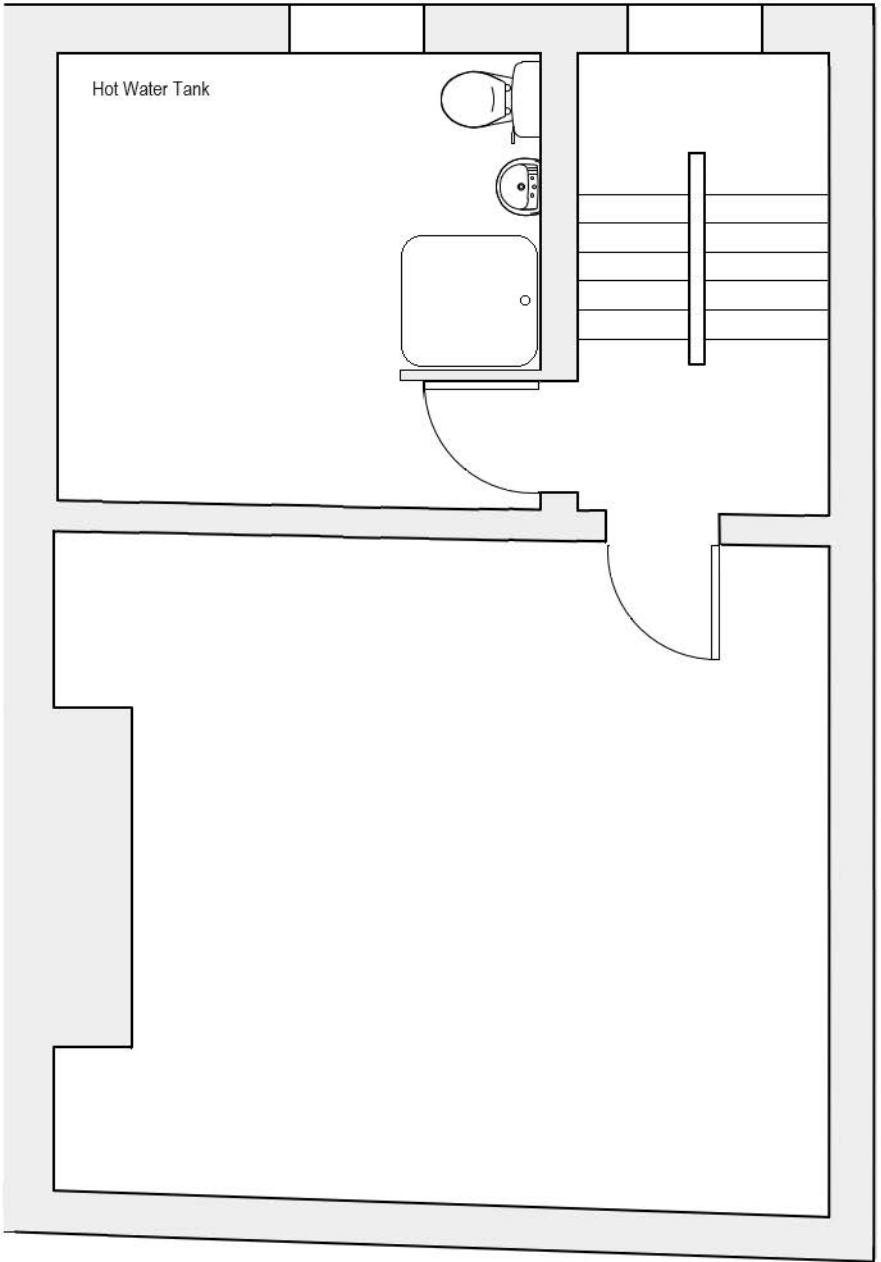
First Floor Plan - Proposed 1:50
