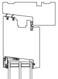
Head Detail 1:5
