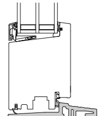
Low-profile Threshold Detail 1:5
