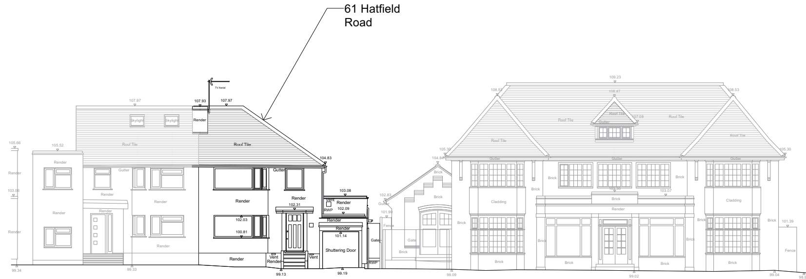
CONTIGUOUS STREETSCAPE WEST ELEVATION
