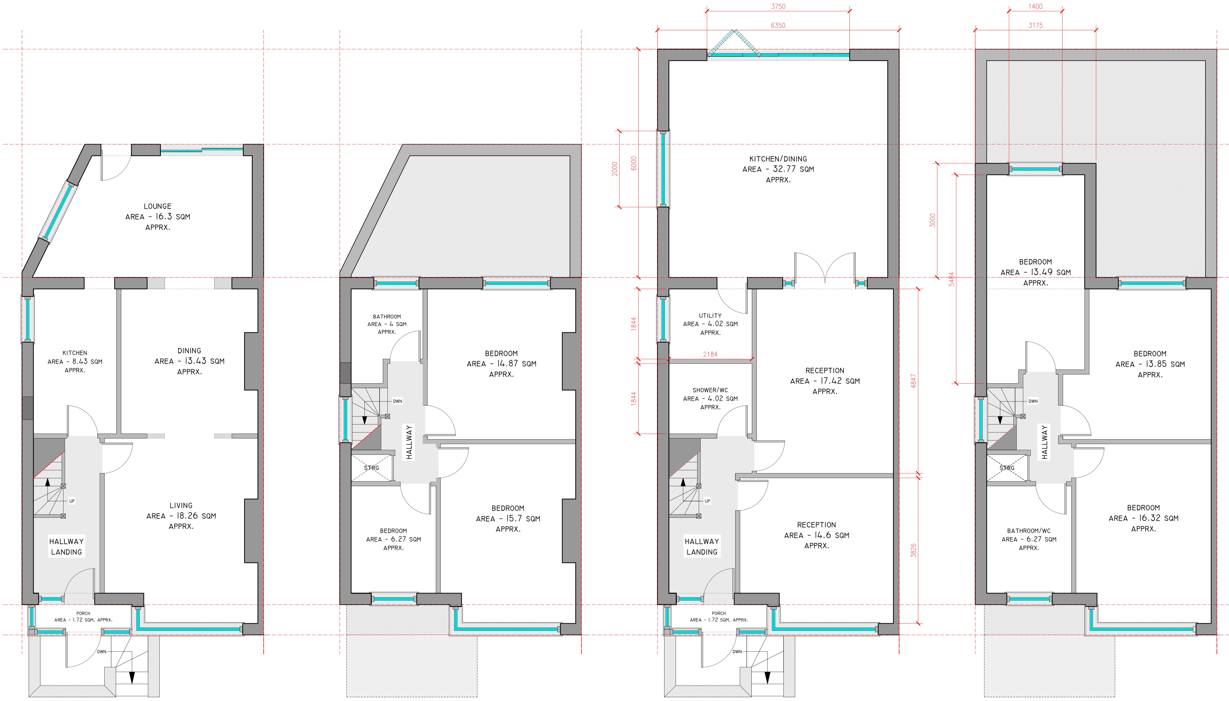
GROUND FLOOR, EXISTING PLAN, SCALE 1:50
