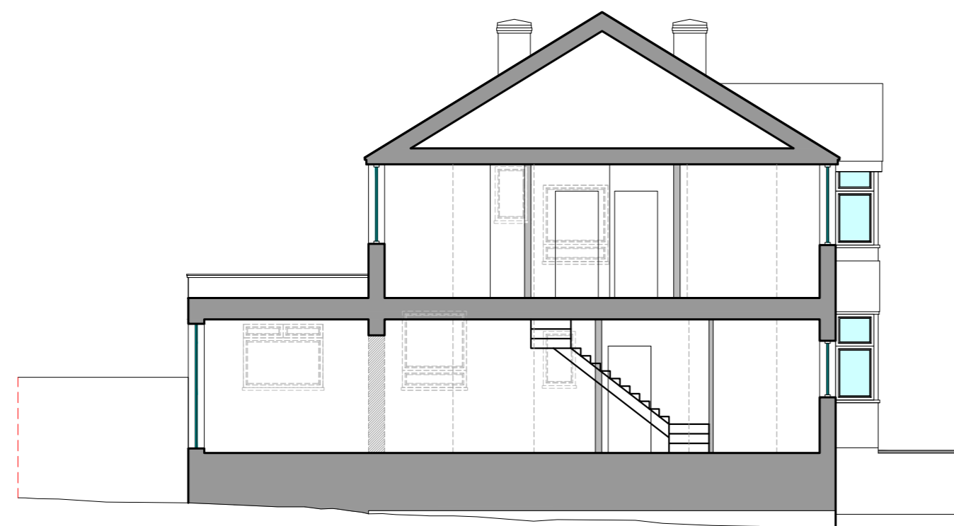
SECTION, EXISTING PLAN, SCALE 1:100
