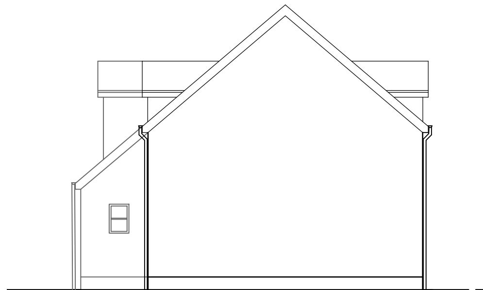
03 | North Elevation 1:100
