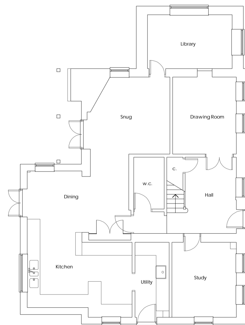
Ground Floor Plan As Proposed (Unchanged)
