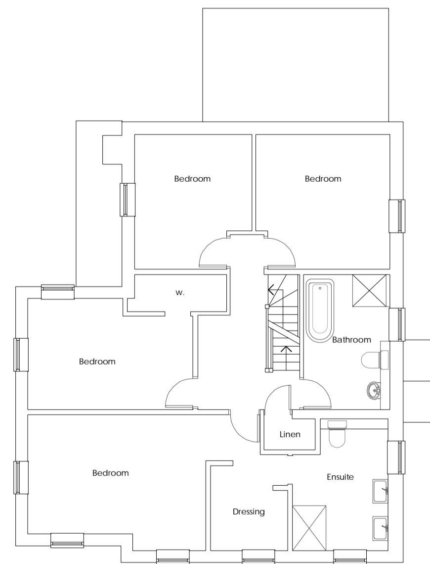
First Floor Plan As Proposed (Unchanged)
