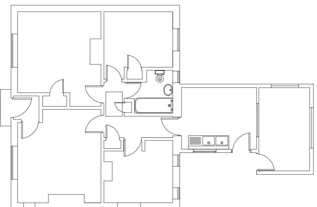
EXISTING GROUND FLOOR PLAN 1:50 @ A1
