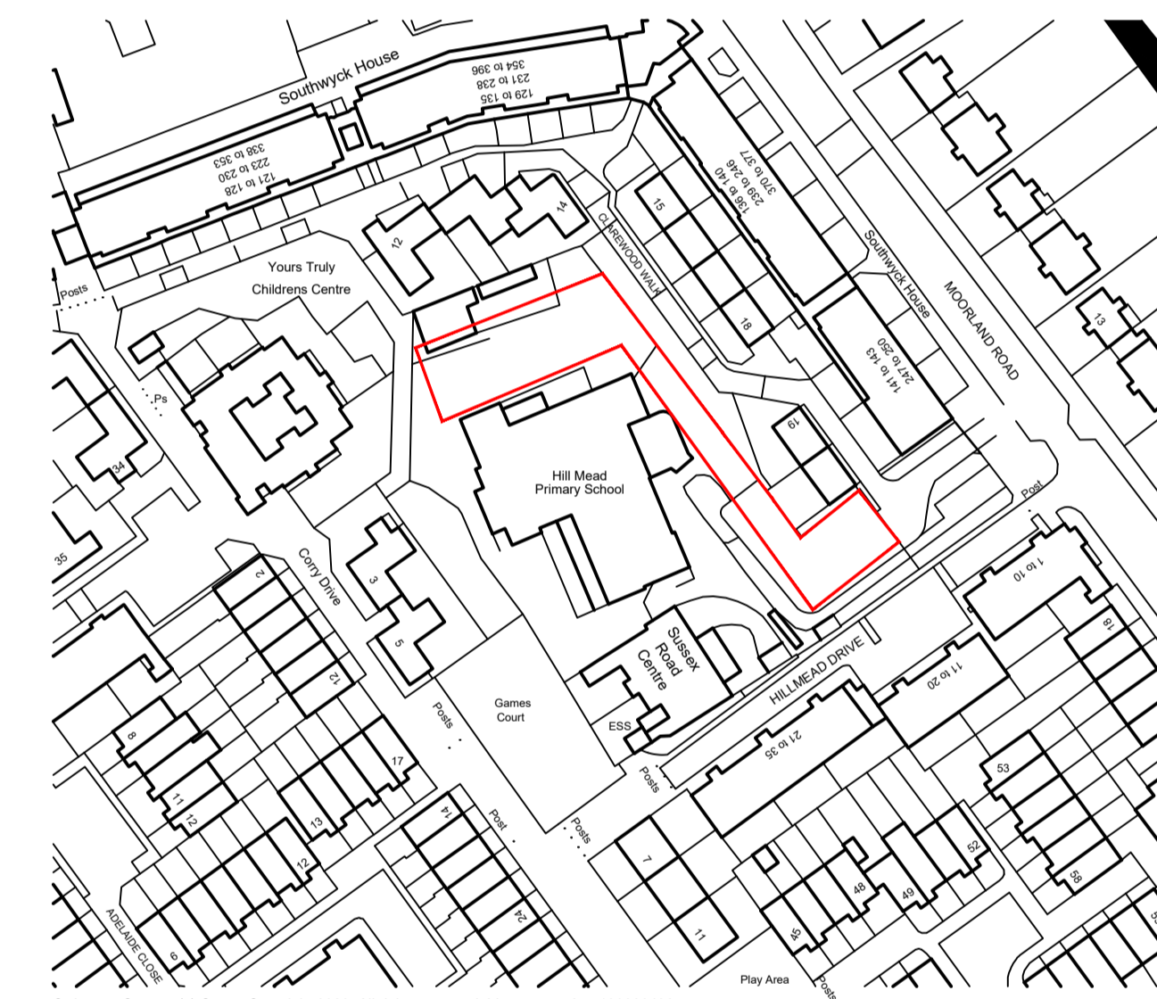
LOCATION PLAN 0m 20m 40m 60m 1:1250
