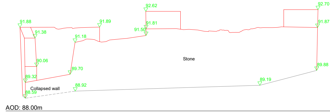
North Elevation
