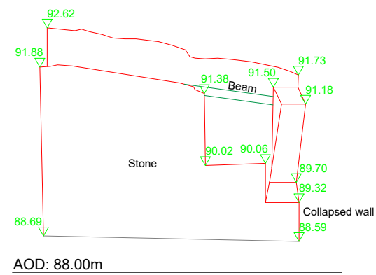
East Elevation
