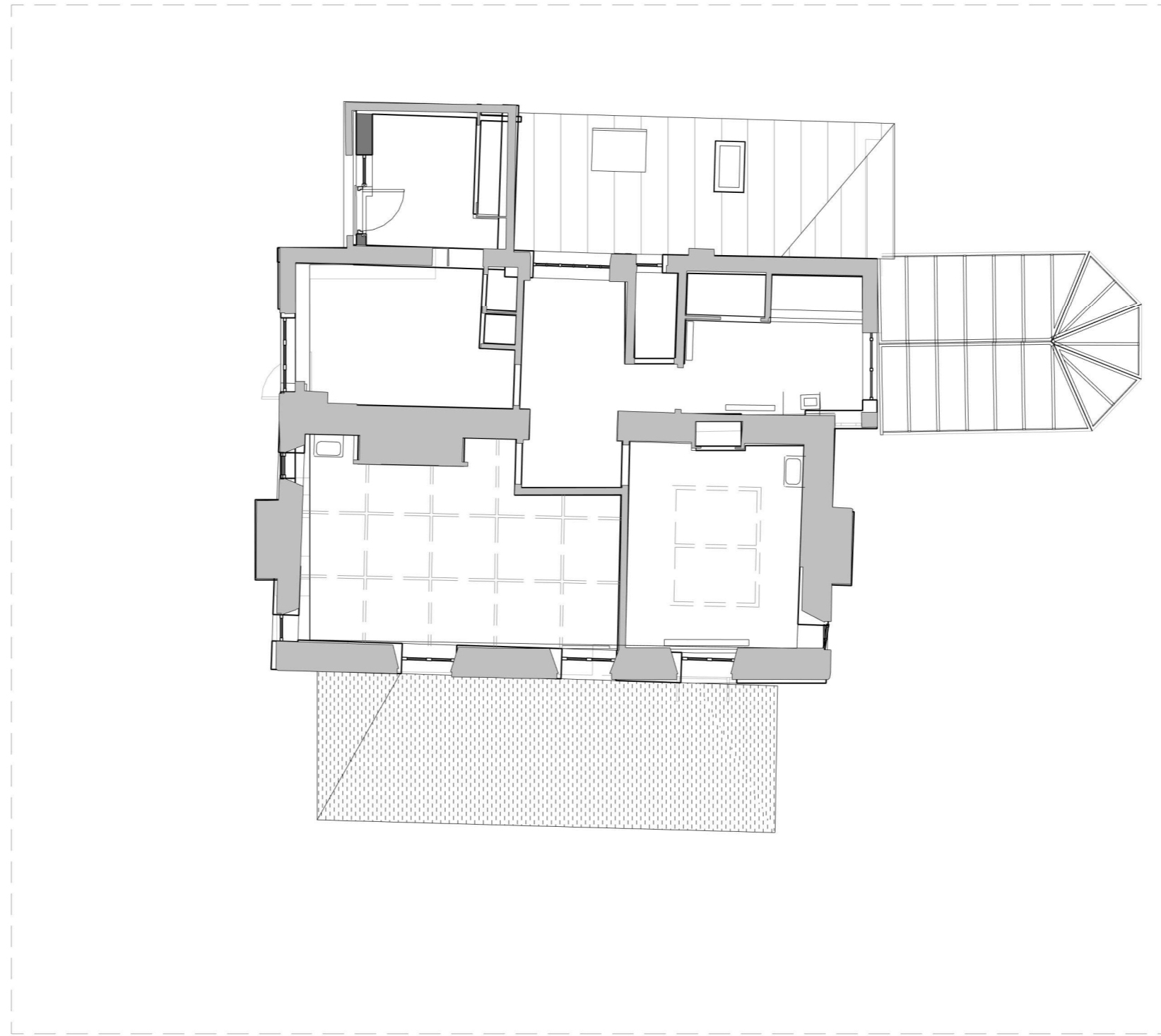
First Floor Plan as Existing 1 : 100
