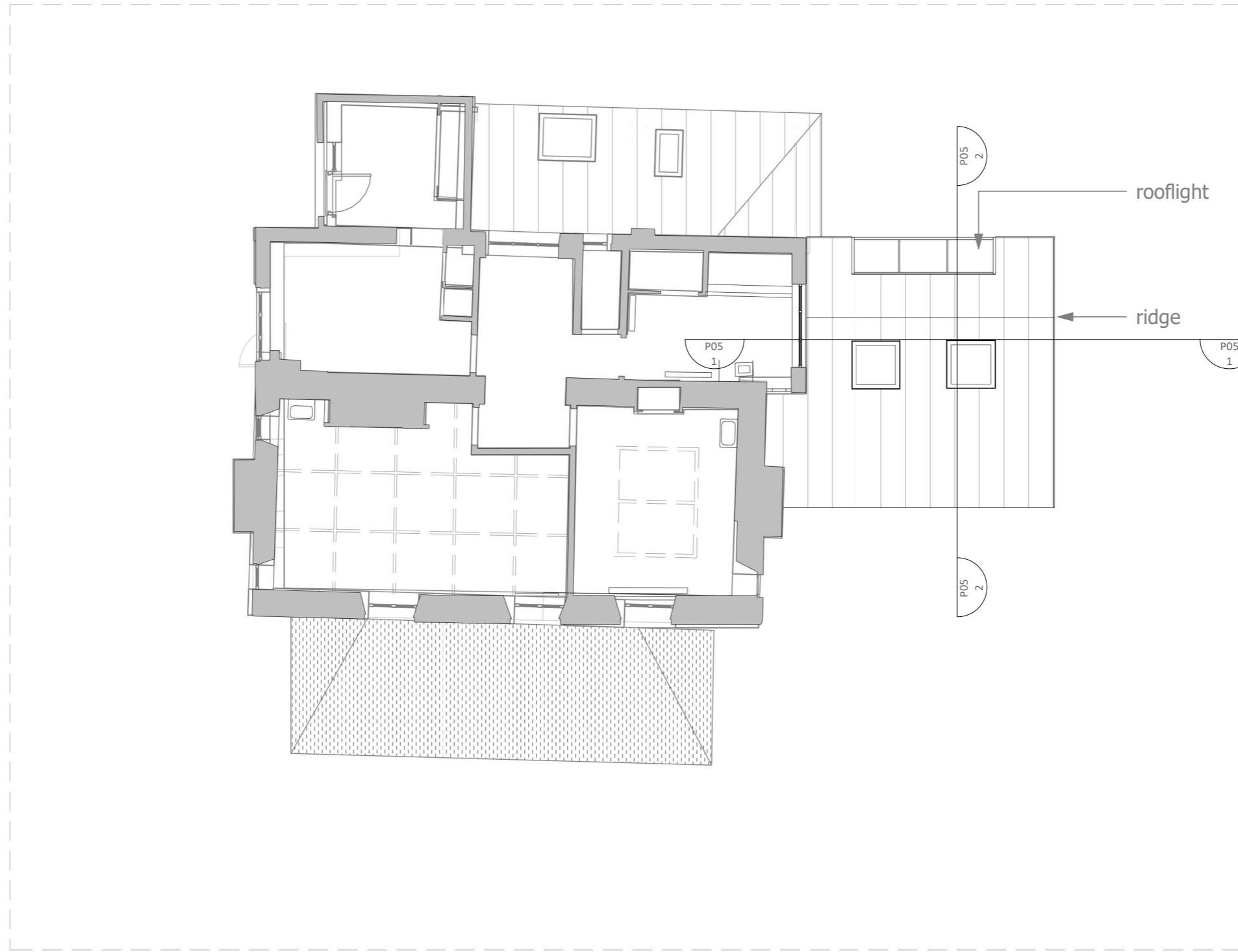
First Floor Plan as Proposed 1 : 100
