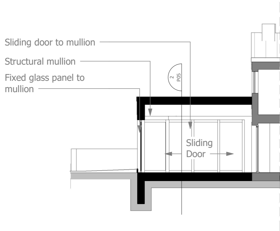
Section AA' as Proposed 1 : 100
