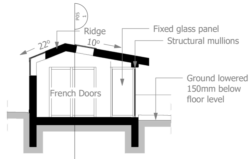
Section BB' as Proposed 1 : 100
