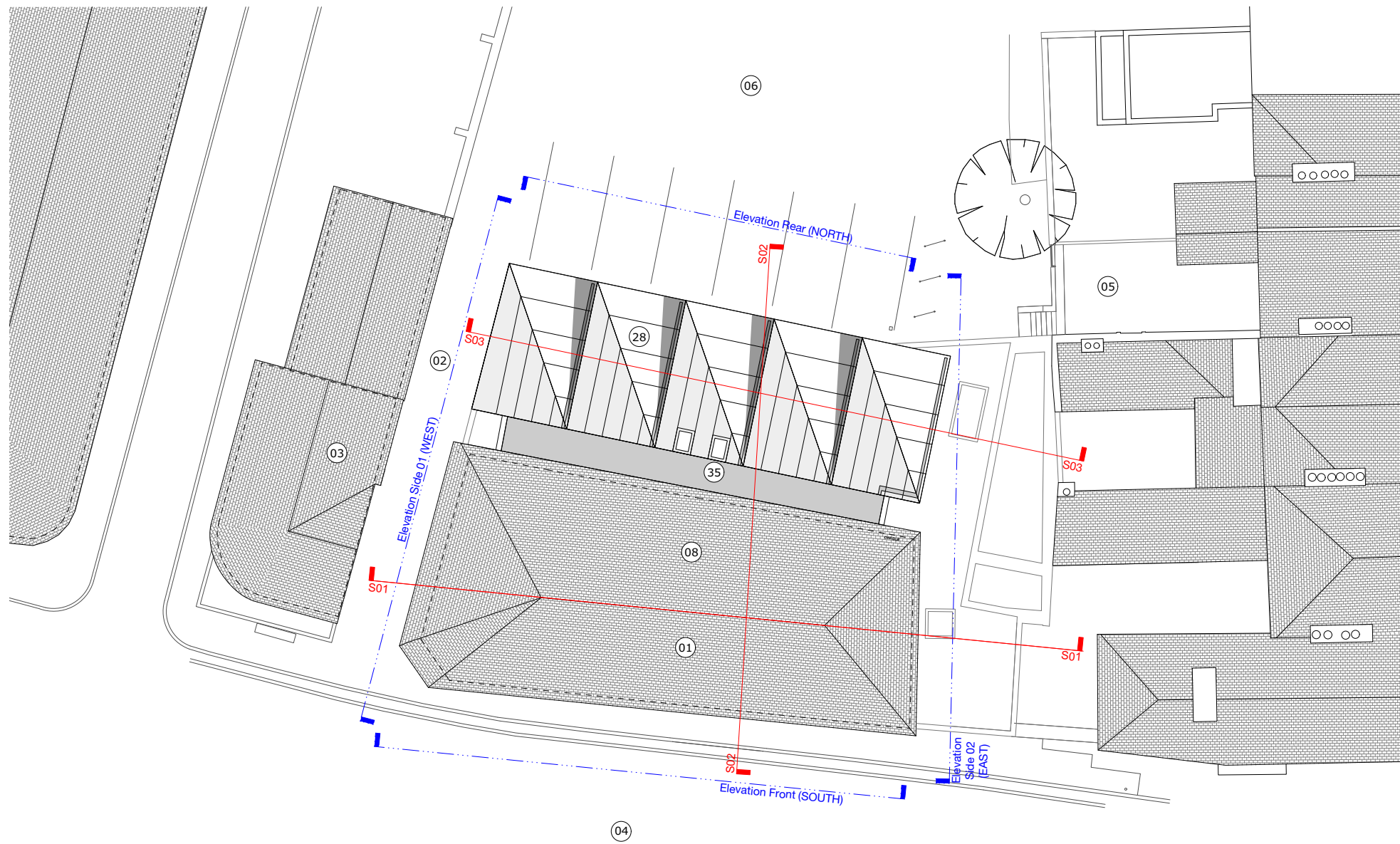
01 PROPOSED SITE PLAN 1:200
