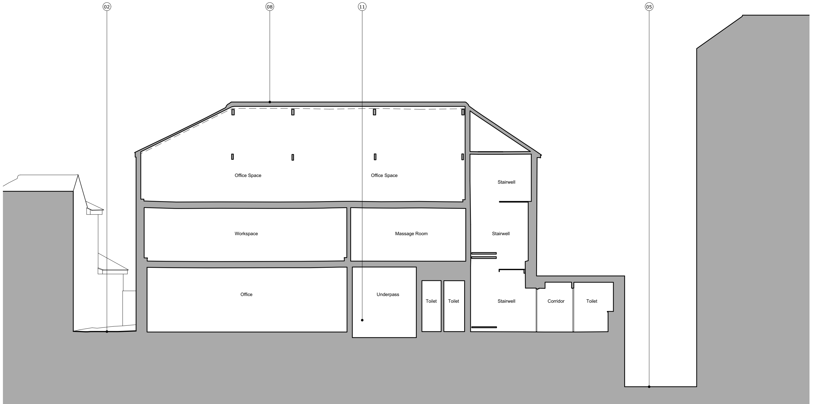
01 EXISTING SECTION 01 1:100
