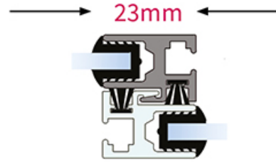
Standard interlock
