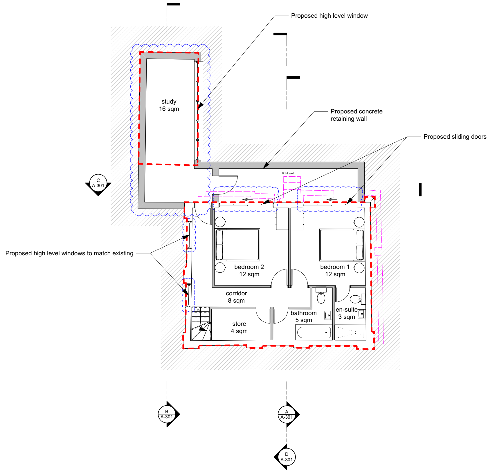
PROPOSED BASEMENT FLOOR PLAN
