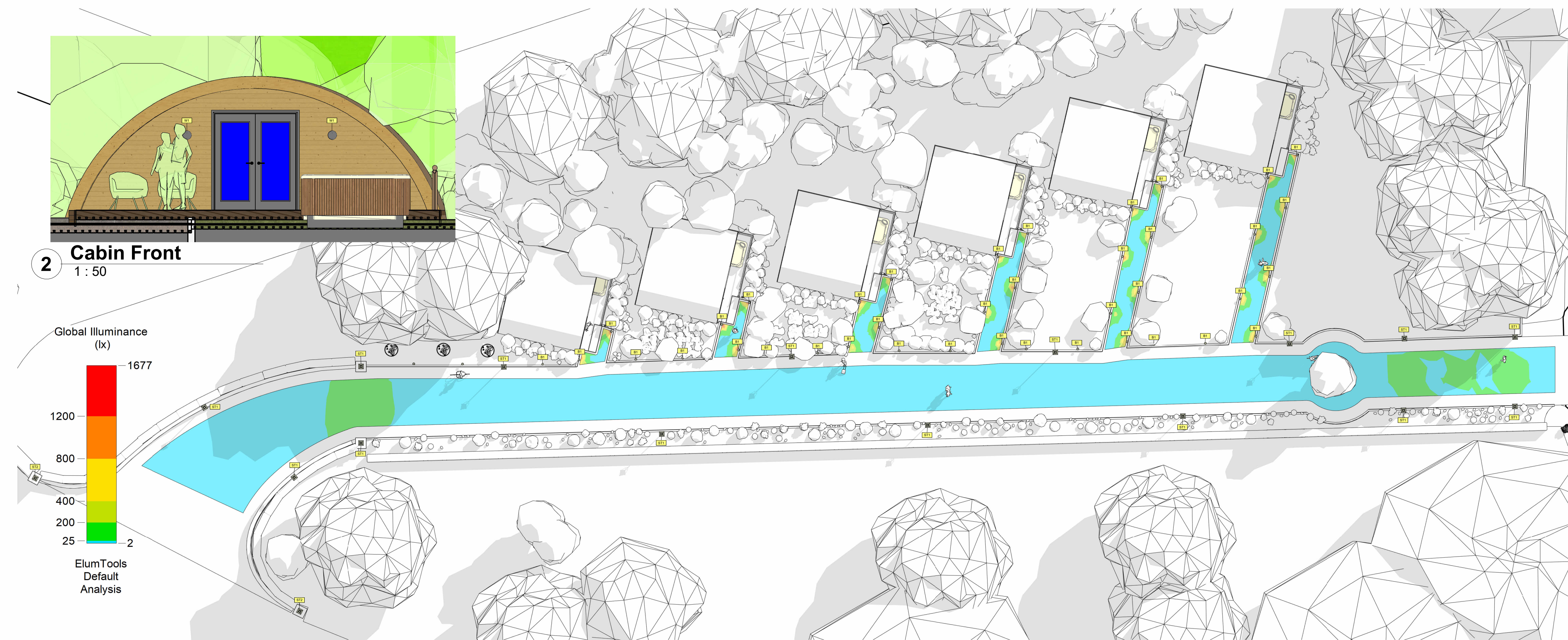
1 External Lighting 1 : 200
