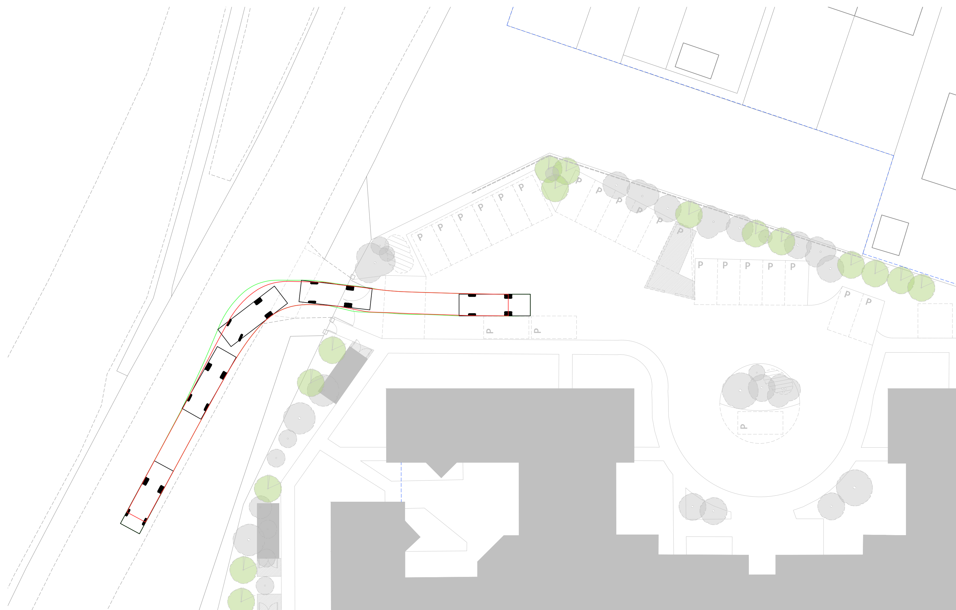
Refuse Vehicle - Exit Scale 1:250
