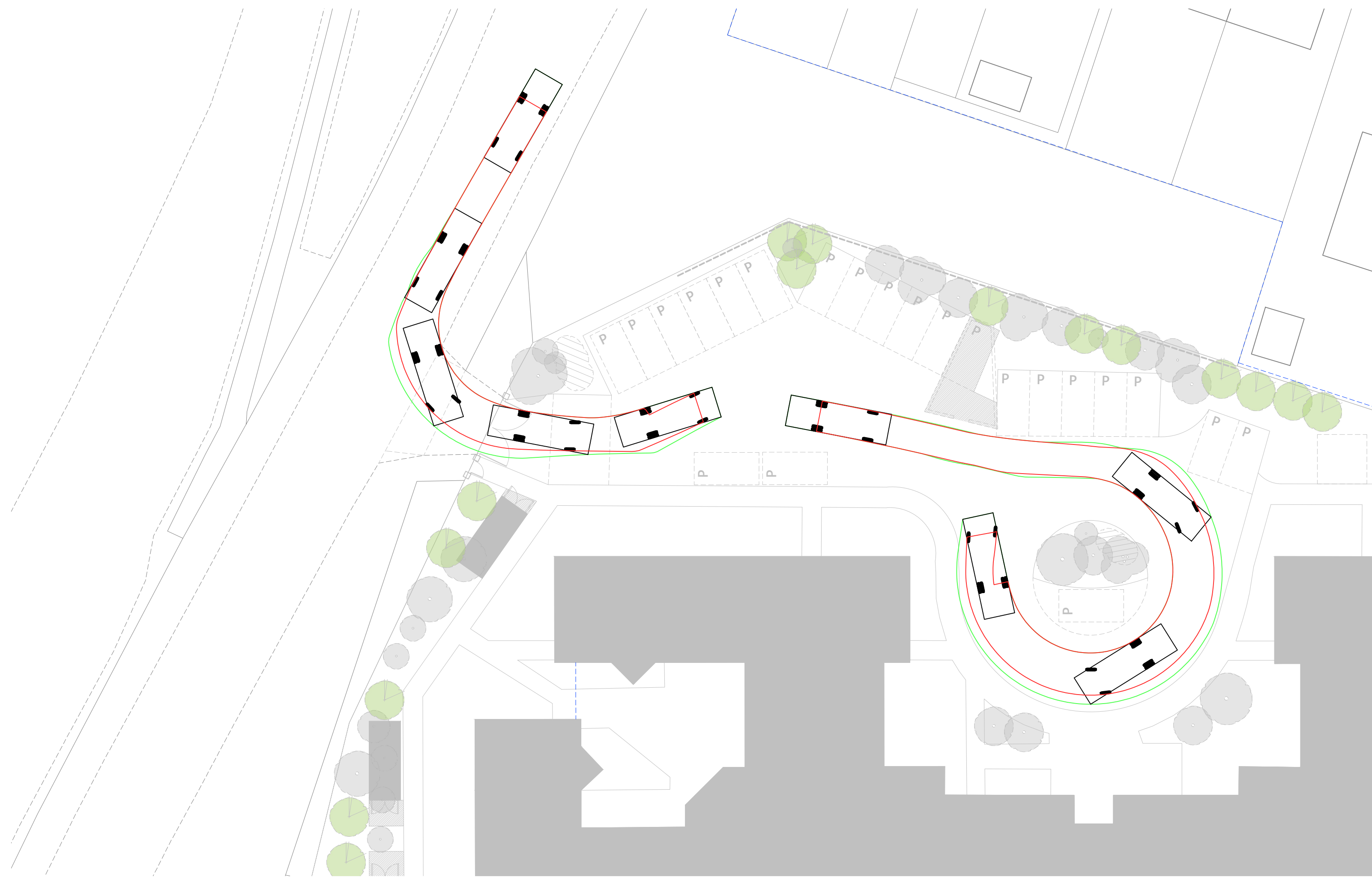
Refuse Vehicle - Entry and Turning Scale 1:250
