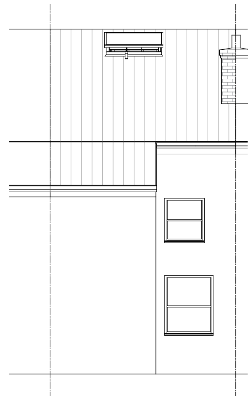
Existing Rear Elevation (South)
