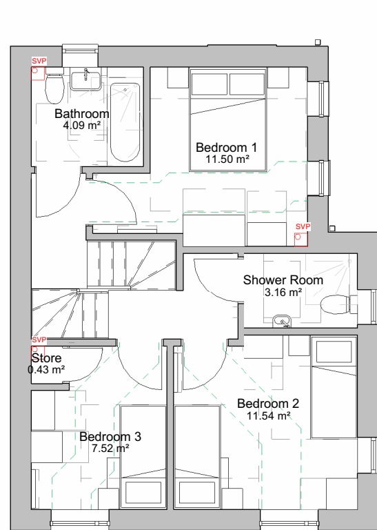
1 First Floor Plan 1 : 100
