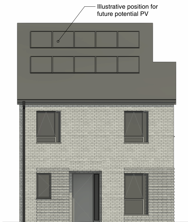
3 Front Elevation 1 : 100
