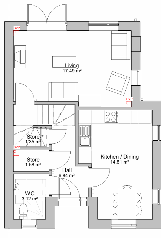
2 Ground Floor Plan 1 : 100
