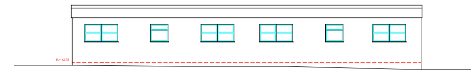
Datum 40.00 Rear Elevation - South East
