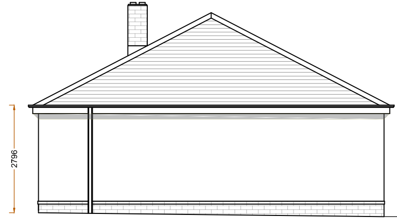
Existing LHS Elevation
