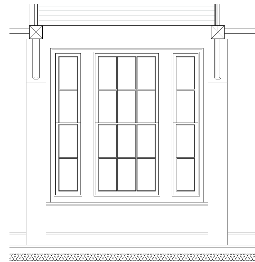
1:20 SCALE INTERNAL ELEVATION OF WG/08
