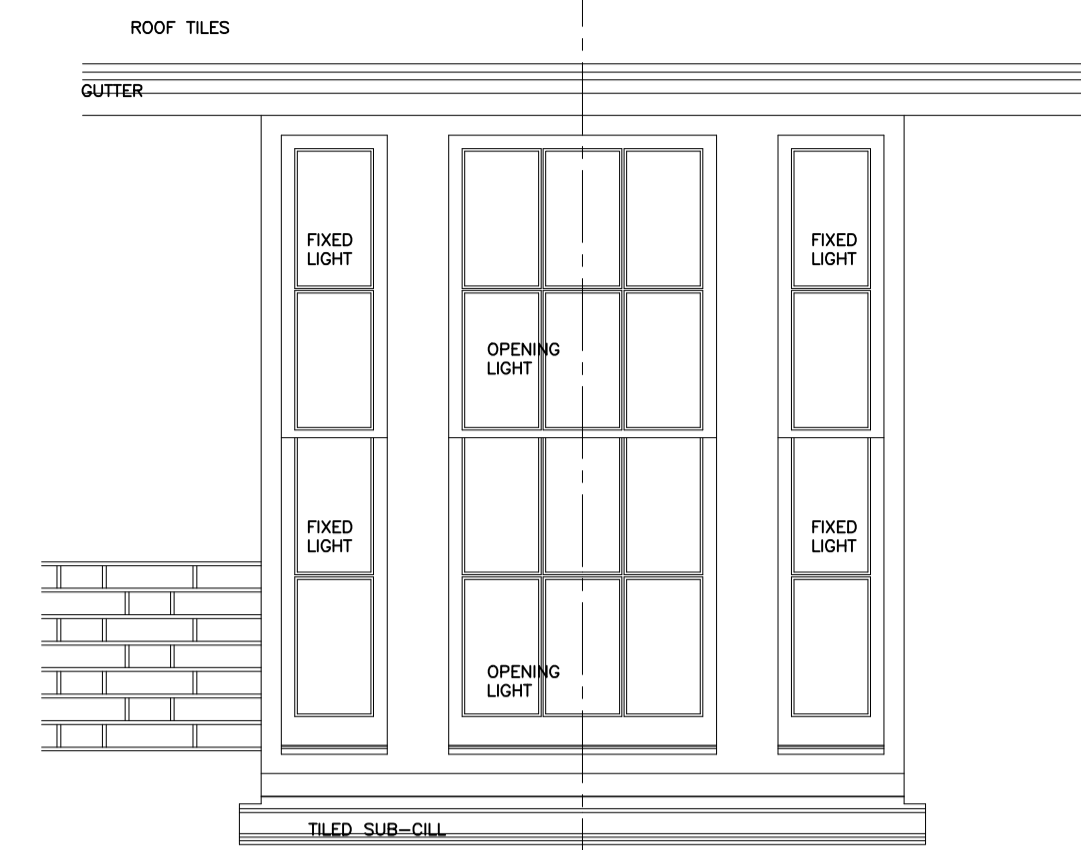
1:20 SCALE ELEVATION OF WG/08
