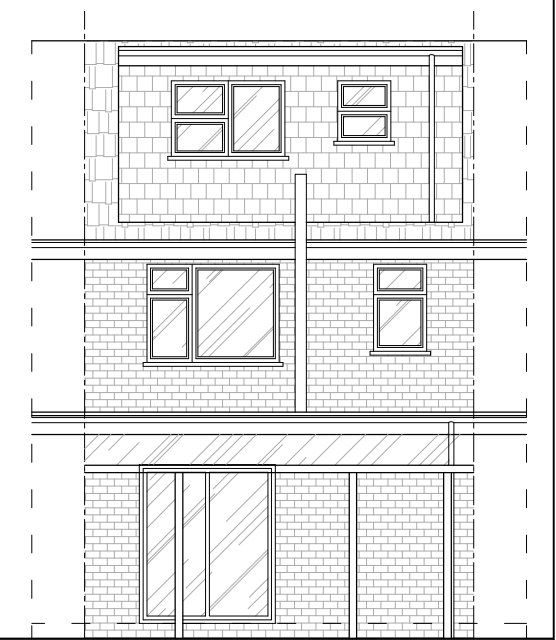
EXISTING / PROPOSED REAR ELEVATION
