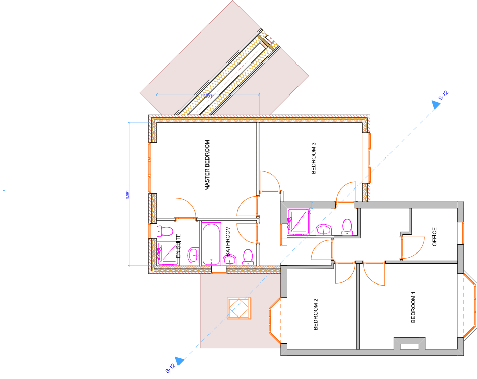
01-First Floor 1:100
