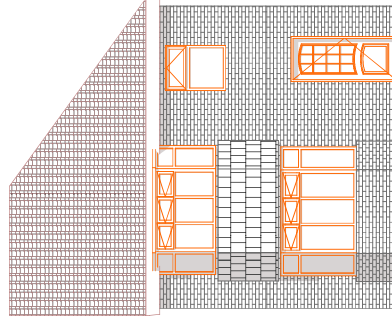
3 - E-South Elevation 1:100
