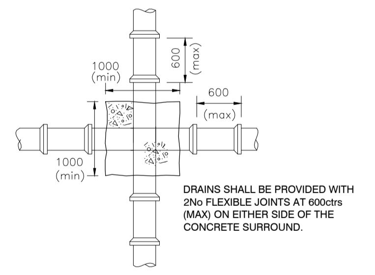
Plan On Pipe Crossover
