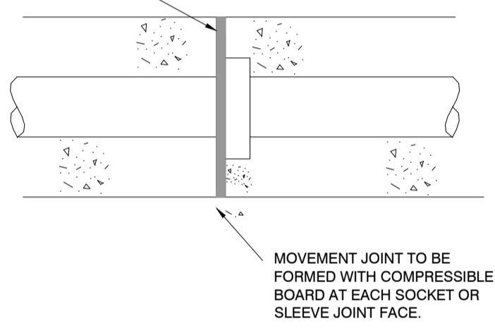
MOVEMENT JOINT TO CONCRETE PIPE SURROUND
