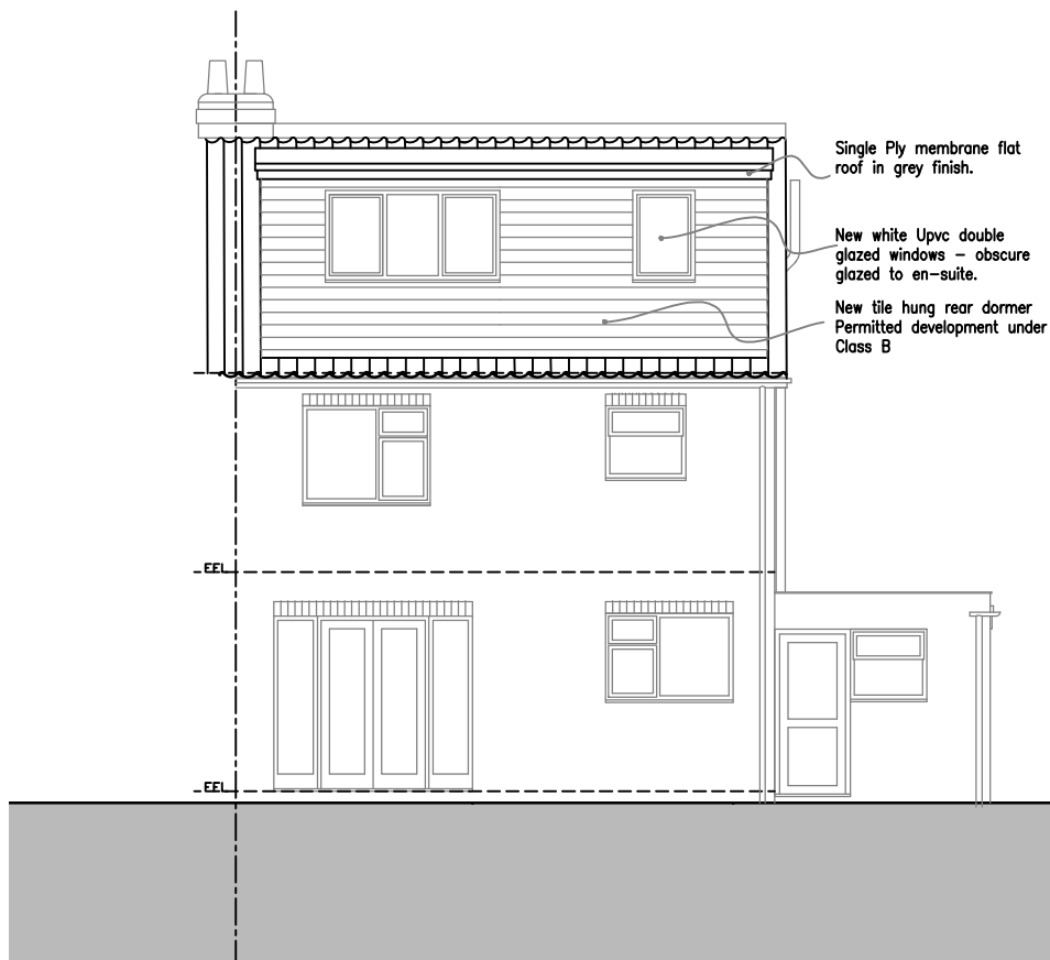
Rear West Facing Elevation
