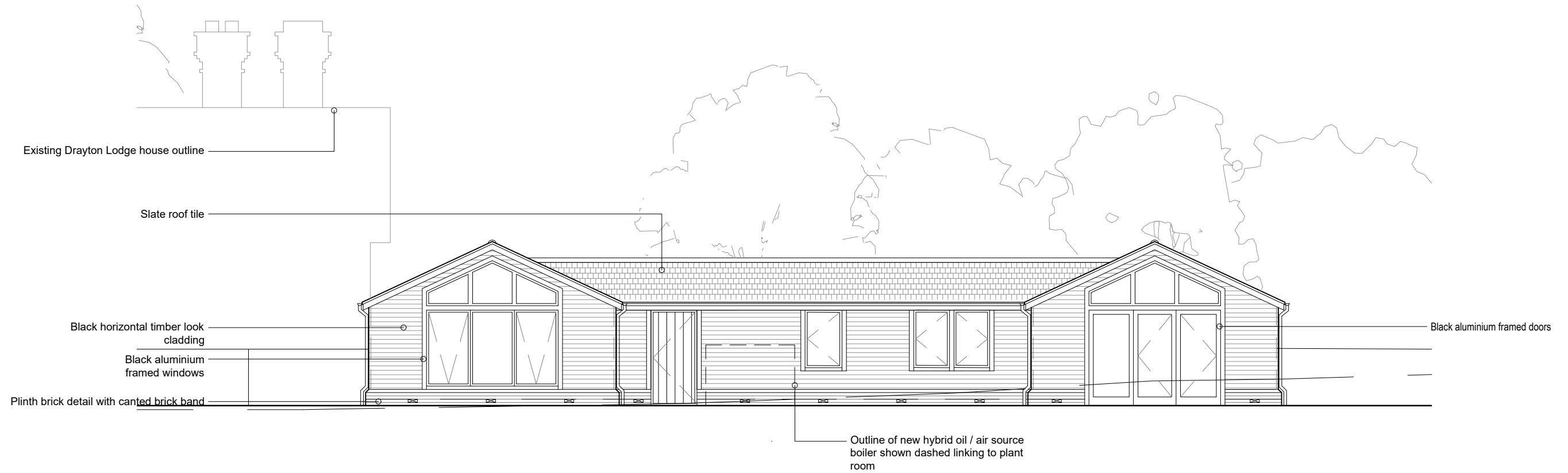
01 PROPOSED SOUTH WEST ELEVATION 105 1:100
