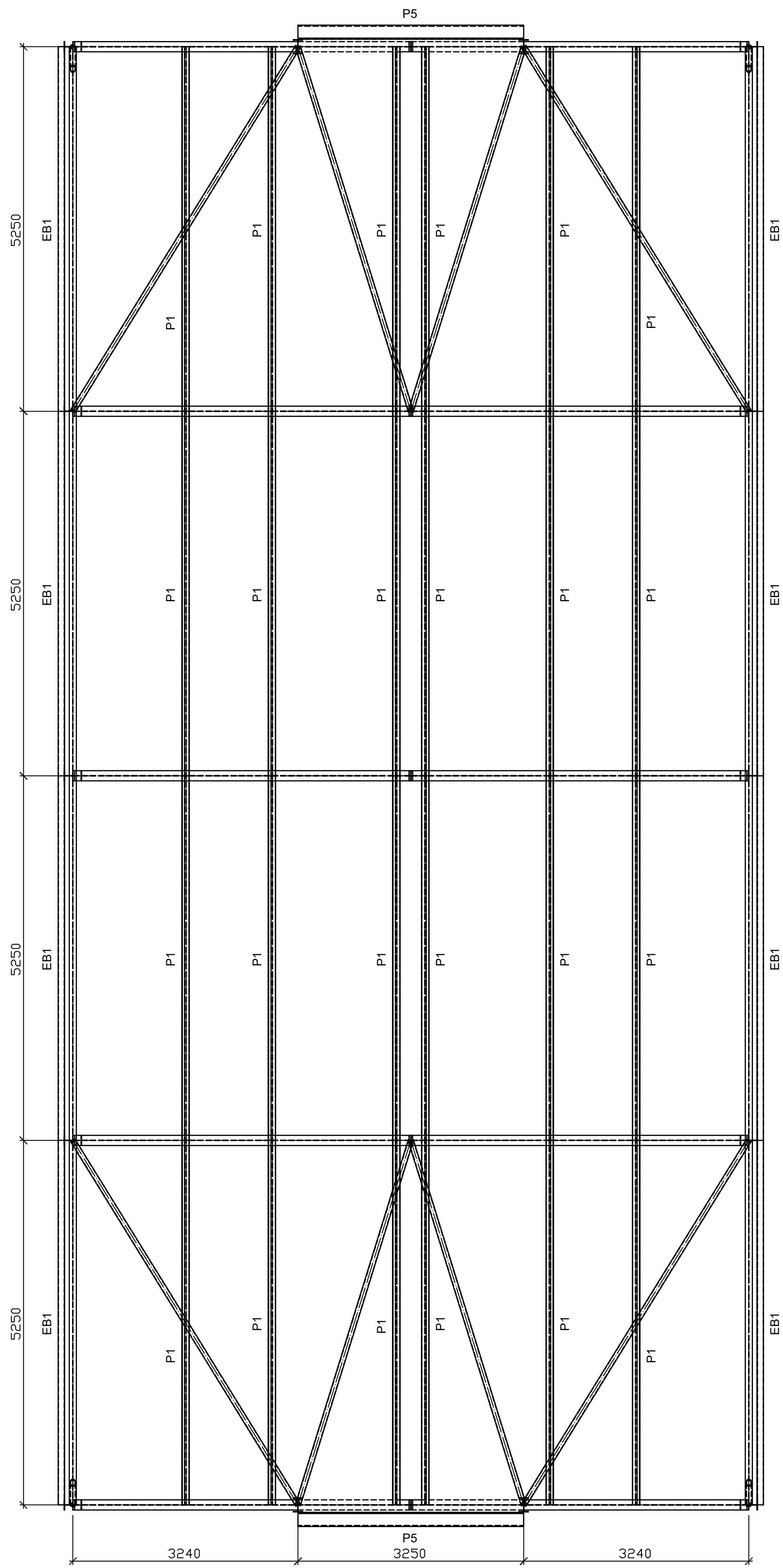
Cold Rolled Roof Plan PLAN ON ROOF
