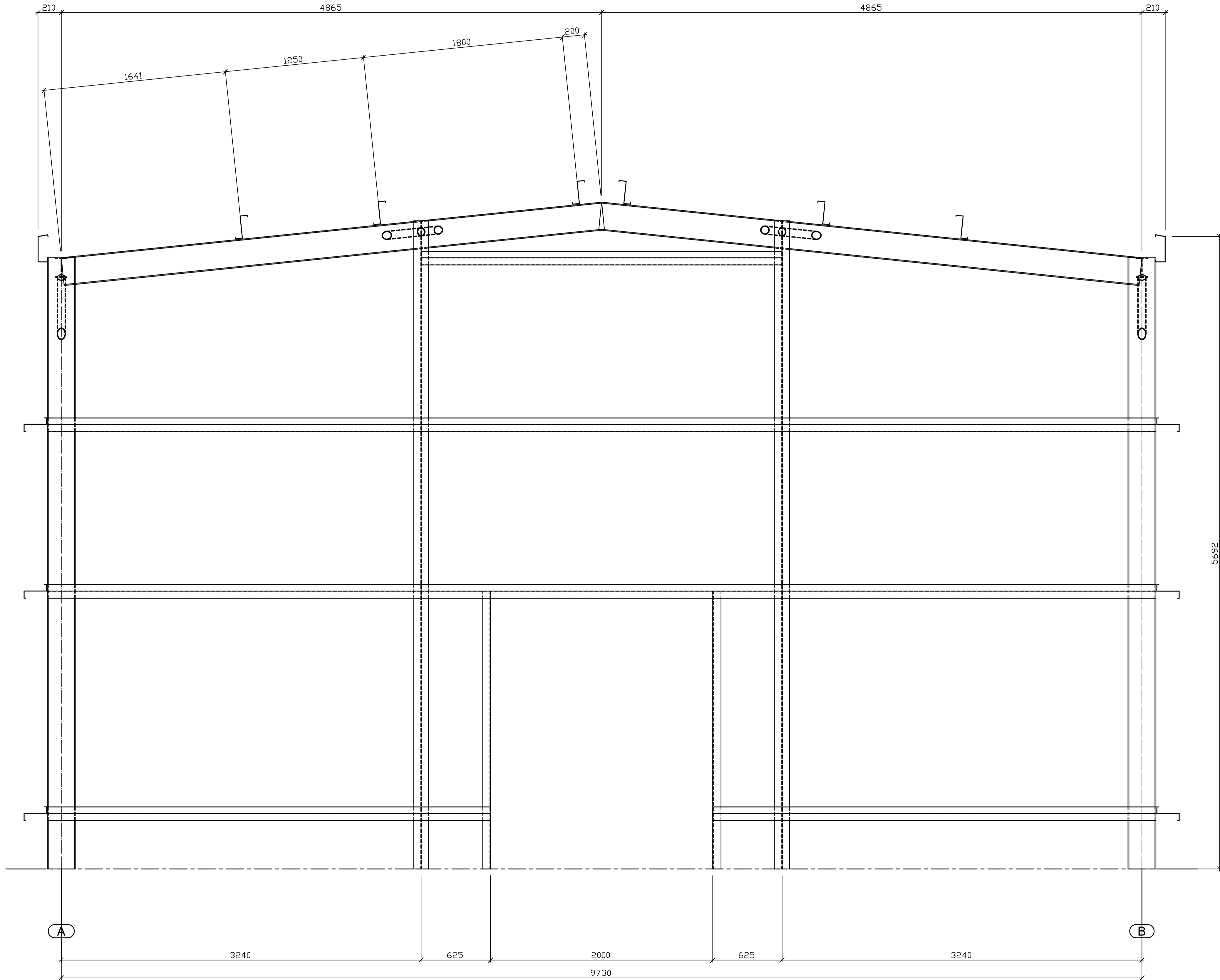
Cold Rolled Elevation on VIEW ON LINE 1 (LINE 5 SIMILAR)
