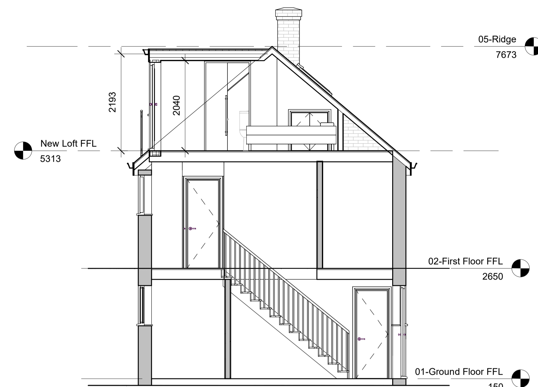
1 Section 1 1 : 50 VISUAL SCALE 1:50 @ A1
