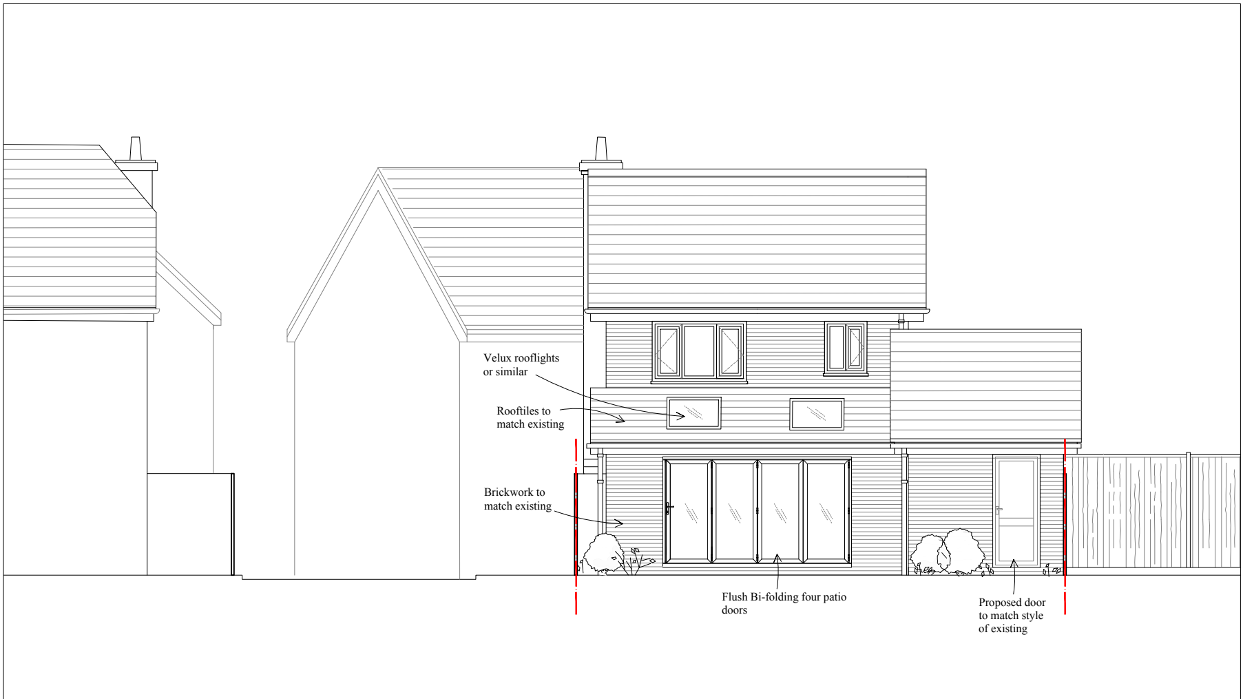
2 WEST ELEVATION 121 AS PROPOSED
